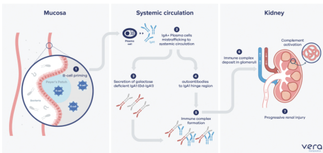
Figure 2: IgAN pathophysiology—overview
